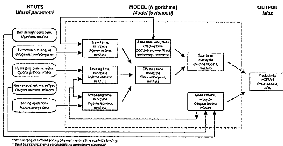
Figure 27. Forwarder productivity model
