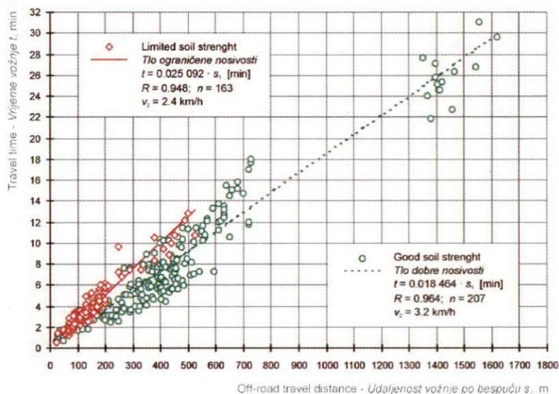
Figure 16. Loaded forwarder (soil strenght conditions)
