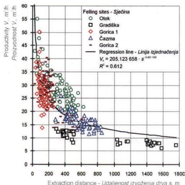
Figure 8. Productivity vs. extraction distance
