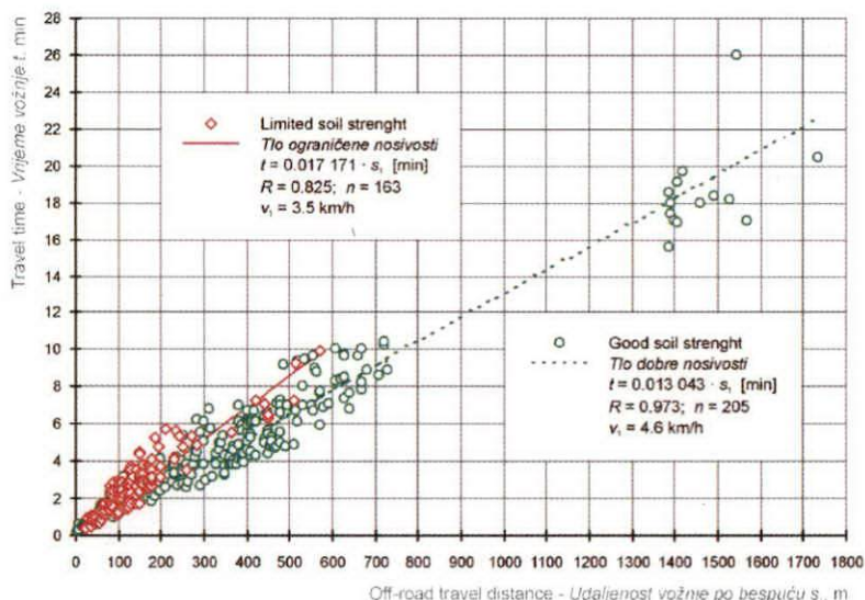
Figure 15. Unloaded forwarder (soil strenght conditions)
