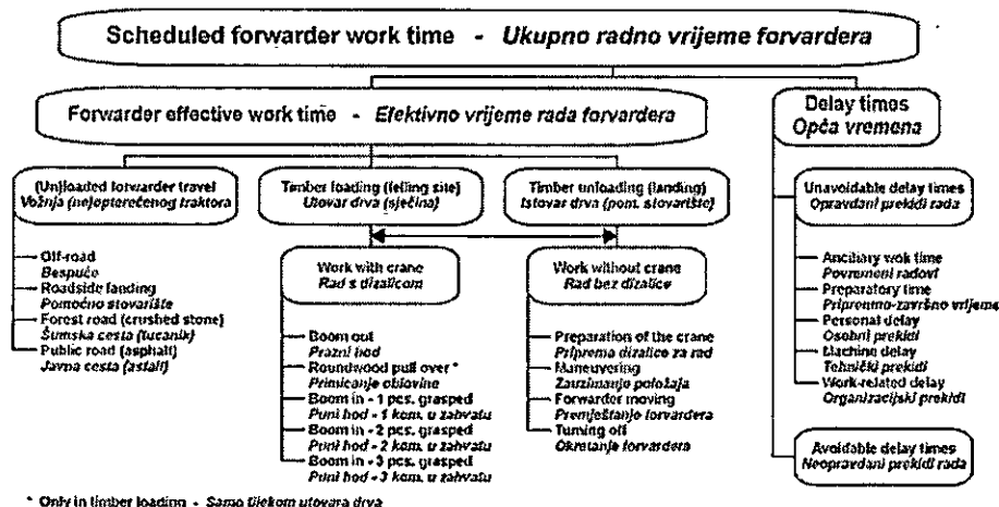
Figure 3. Working components
